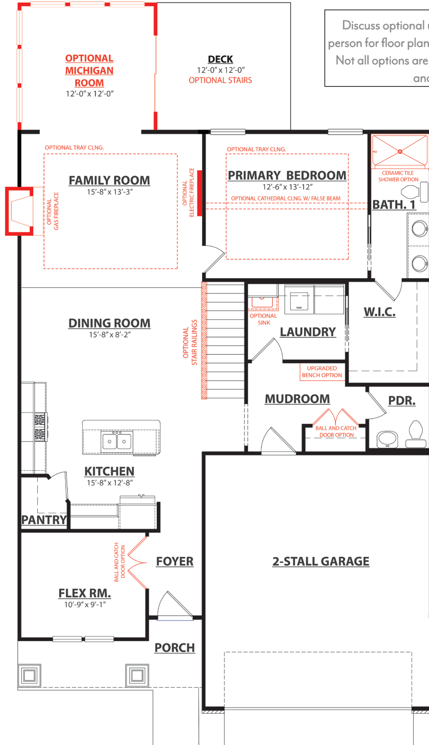
OPTIONAL UPGRADES - FIRST FLOOR PLAN
